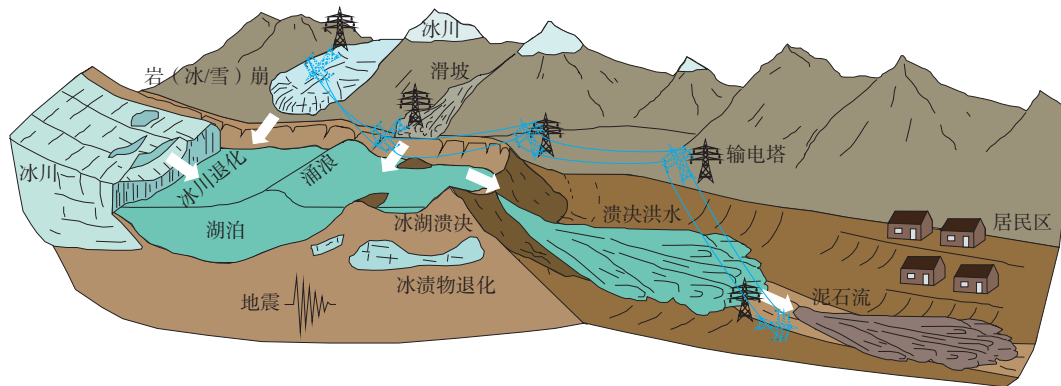
图 15 岩(冰/雪)崩-滑坡-碎屑流-冰湖溃决-洪水-泥石流灾害链演化过程(据 Westoby et al., 2014 修改) Fig. 15 Evolution of the rock (ice/snow)-landslide-debris flow-glacial lake outburst-flood-mudslide hazard chain (modified from Westoby et al., 2014)
